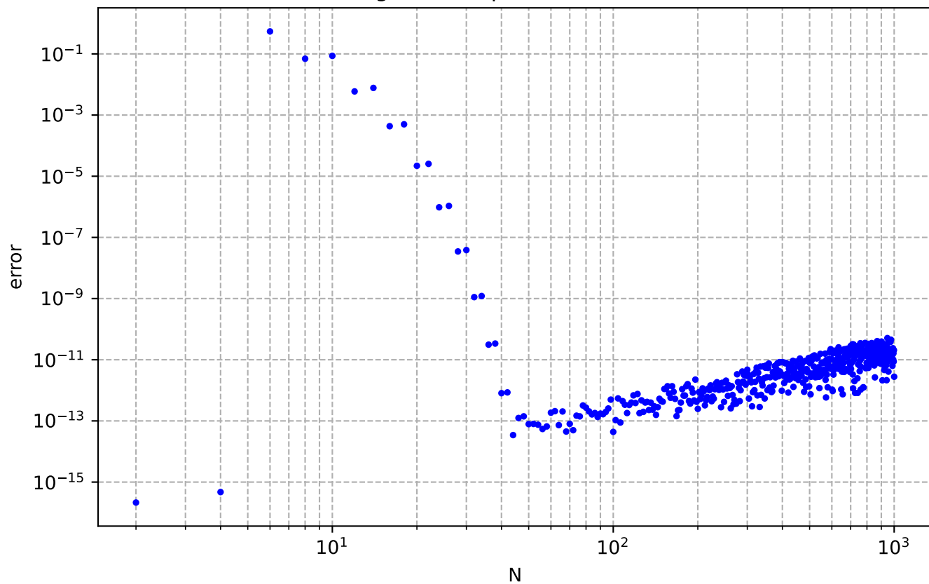
Convergence of spectral differentiation
